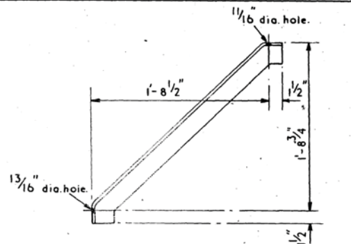
DETAIL 'C' 2\frac{1}{2}'' \times 2\frac{1}{2}'' \times \frac{1}{4}'' M.S. ANGLE
