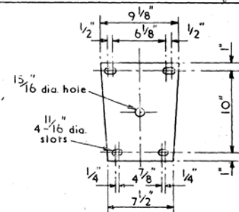
DETAIL 'E' \frac{5}{8}'' M.S. PLATE
