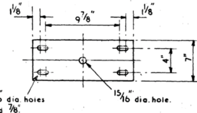
DETAIL 'B' \frac{5}{8}'' M.S. PLATE
