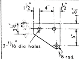
DETAIL 'G' \frac{3}{4}'' W.I. PLATE
