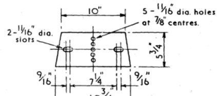
DETAIL 'D' \frac{1}{2}'' M.S. PLATE
