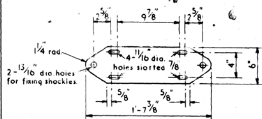
DETAIL 'A' \frac{5}{8}'' M.S. PLATE
