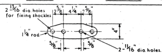
DETAIL 'F' \frac{5}{8}'' M.S. PLATE
