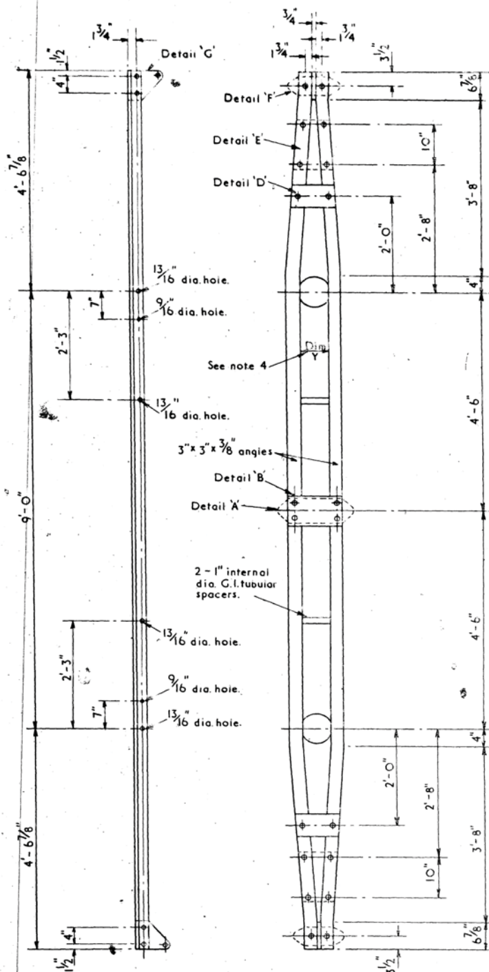
ARRANGEMENT OF CROSSARMS.
